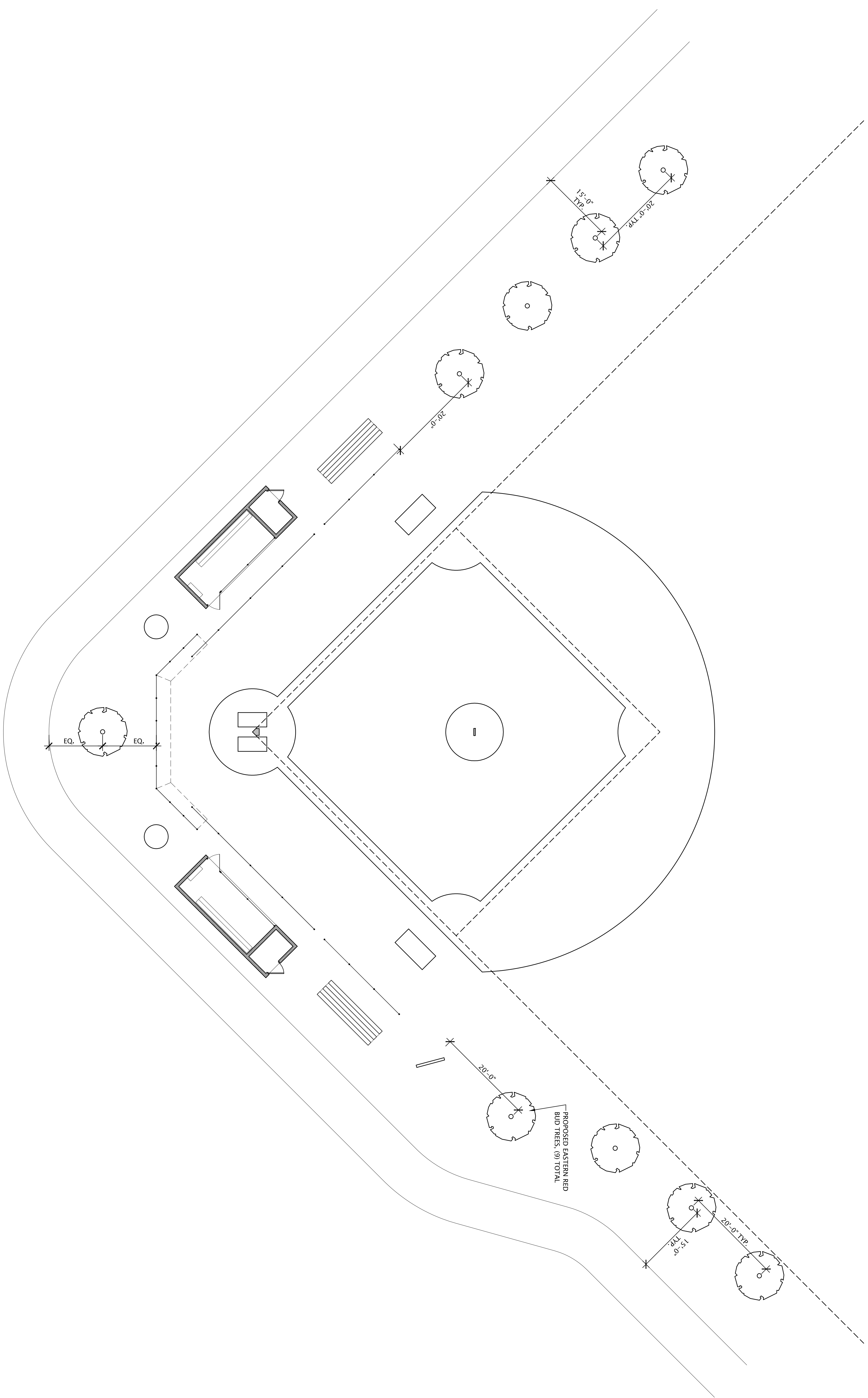
PROPOSED LANDSCAPE PLAN SCALE: 1" = 10'
